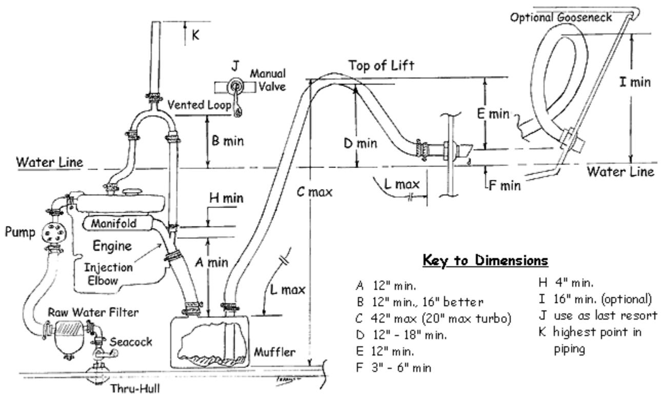
Figure Four: Dimensions
